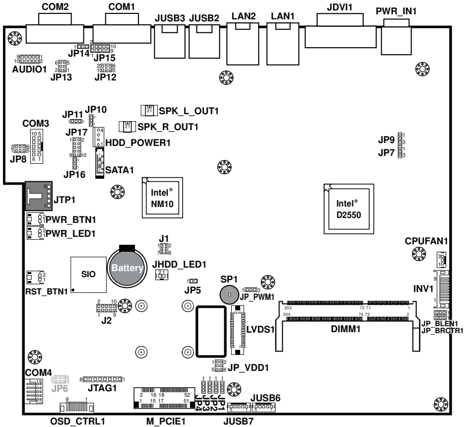
SP-7117 Connectors, Jumpers and Component Locations
