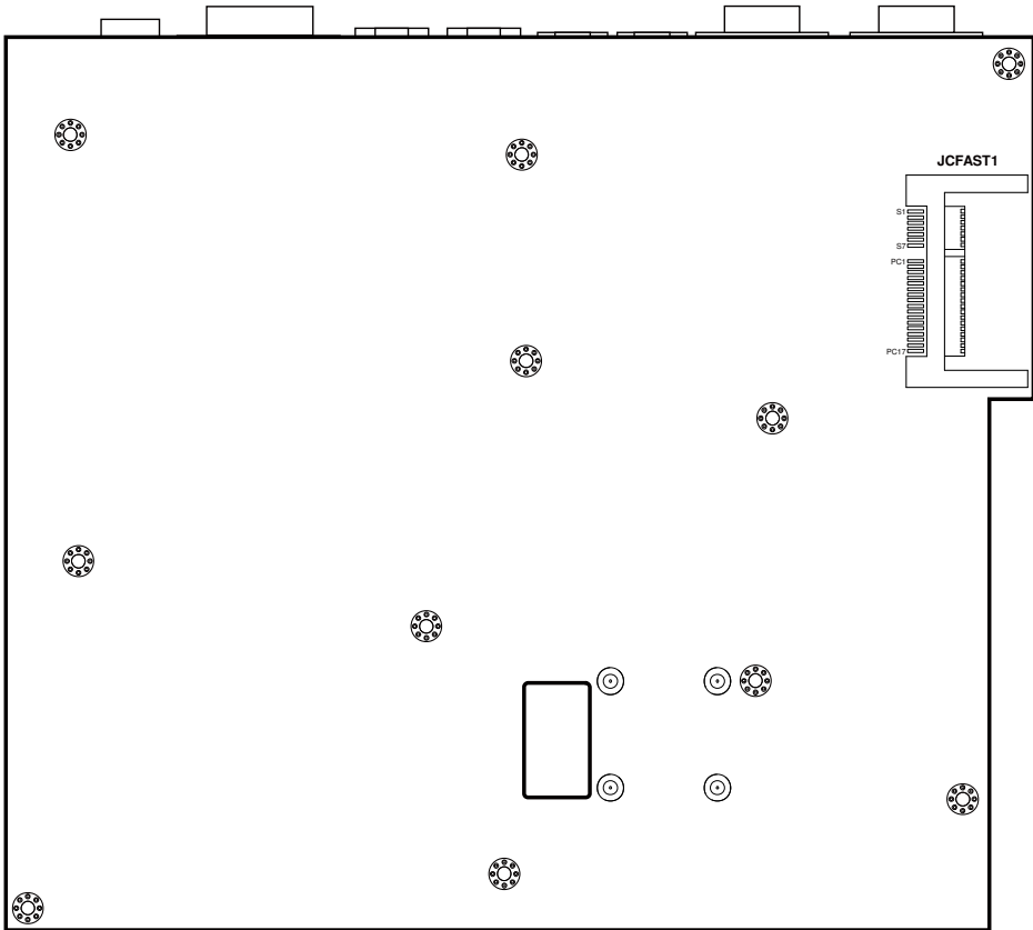
SP-7117 Component Location
