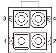
ATX_PWR1
