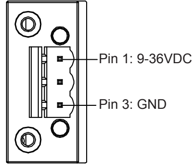
DC IN
