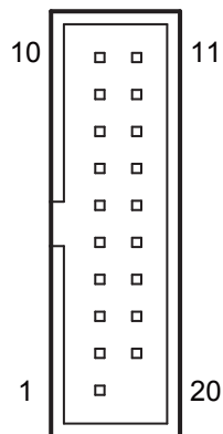
USB1
