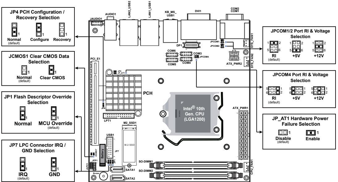
Figure 3-1. BM-D025 Component Location (Top View)
