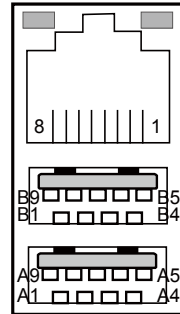
LAN_USB1
